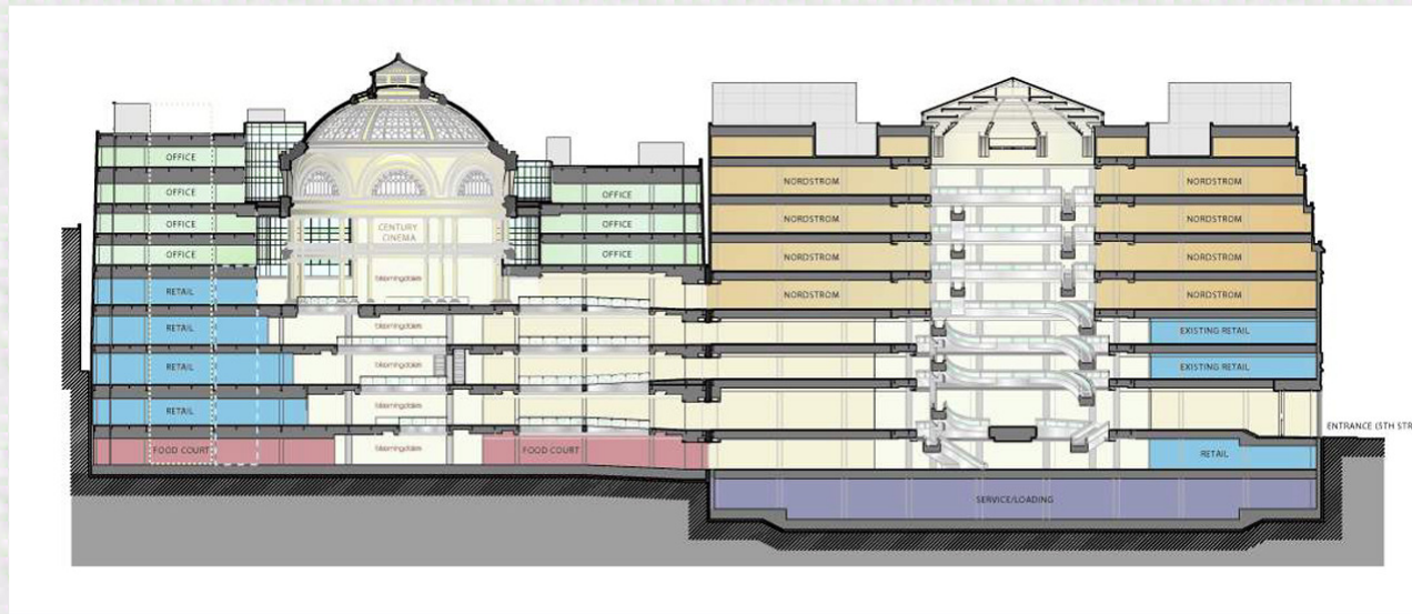
San Francisco Emporium Remodel - San Francisco, California
